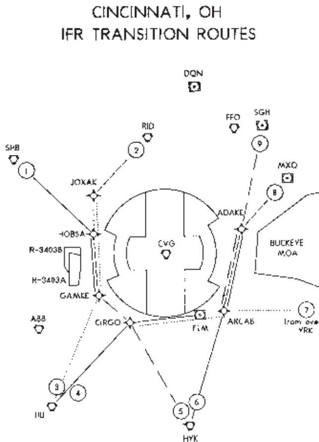
Figure 10. RNAV IFR Terminal Transition Routes
