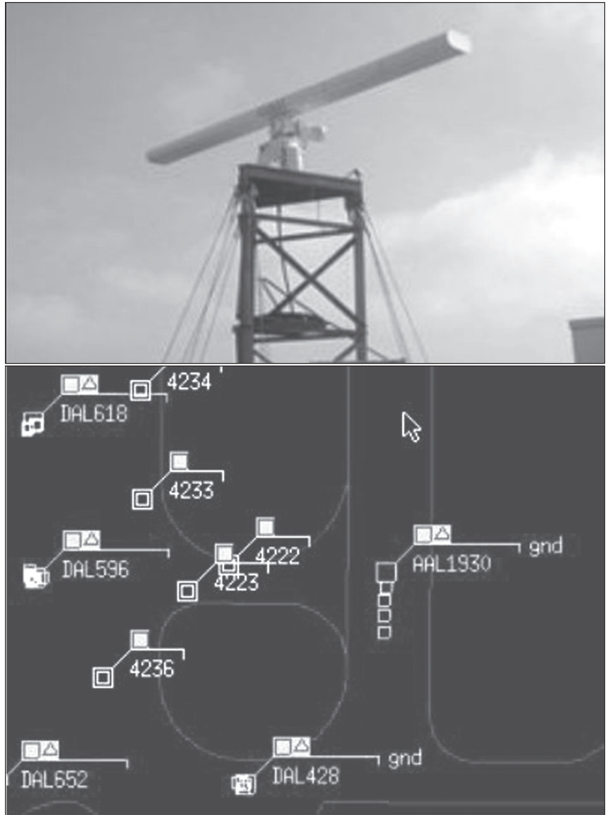
An ASDE radar antenna (top) sweeps 360 degrees per second. Multi Sensor Data Processing (above), a fused view from multiple sensors, showing aircraft and gates.
